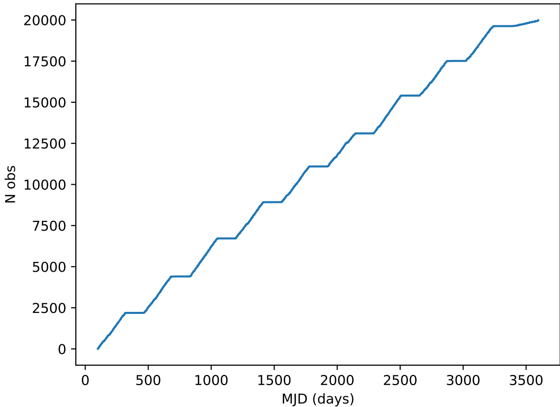
ddf_loaded_half_fl4_v3.4_10yrs all bands: DD:EDFS Cumulative NVisits
