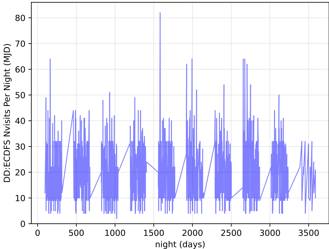
ddf_loaded_half_fl4_v3.4_10yrs all bands: DD:ECDFS Nvisits Per Night
