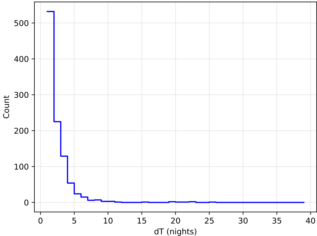
ddf_loaded_half_fl4_v3.4_10yrs all bands: DD:ECDFS Delta Nights Histogram
