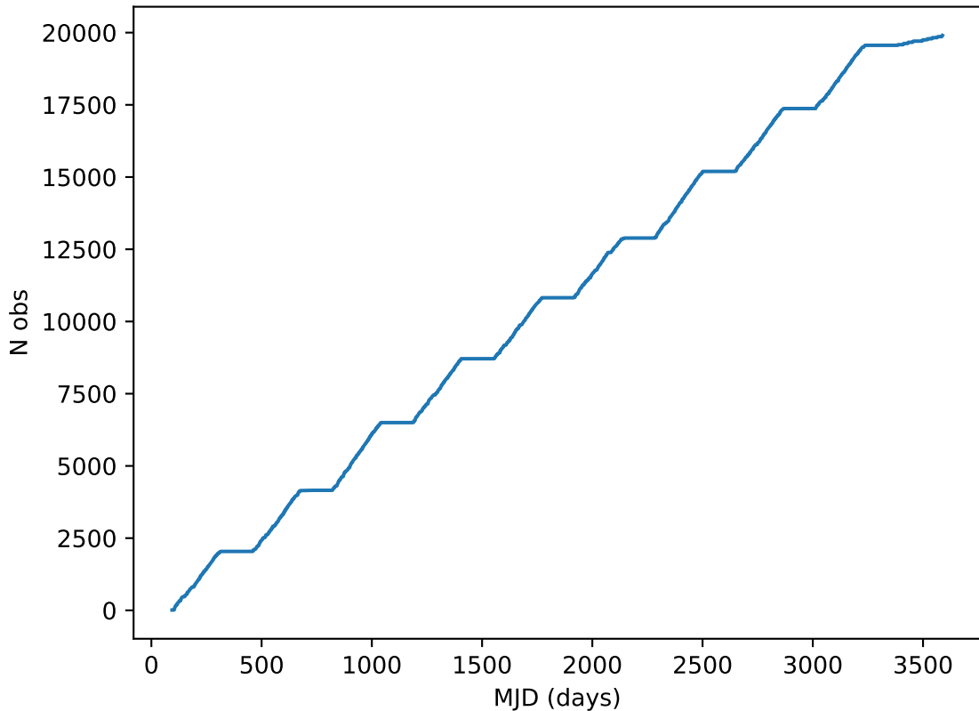
ddf_loaded_half_f14_v3.4_10yrs all bands: DD:ECDFS Cumulative NVisits
