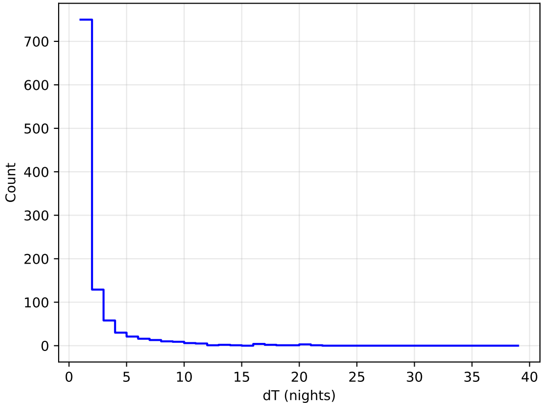
ddf_loaded_half_fl4_v3.4_10yrs all bands: DD: COSMOS Delta Nights Histogram
