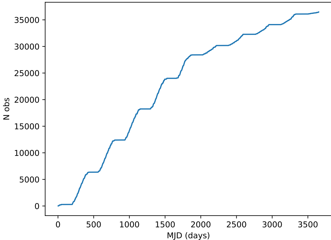
ddf_loaded_half_fl4_v3.4_10yrs all bands: DD:COSMOS Cumulative NVisits
