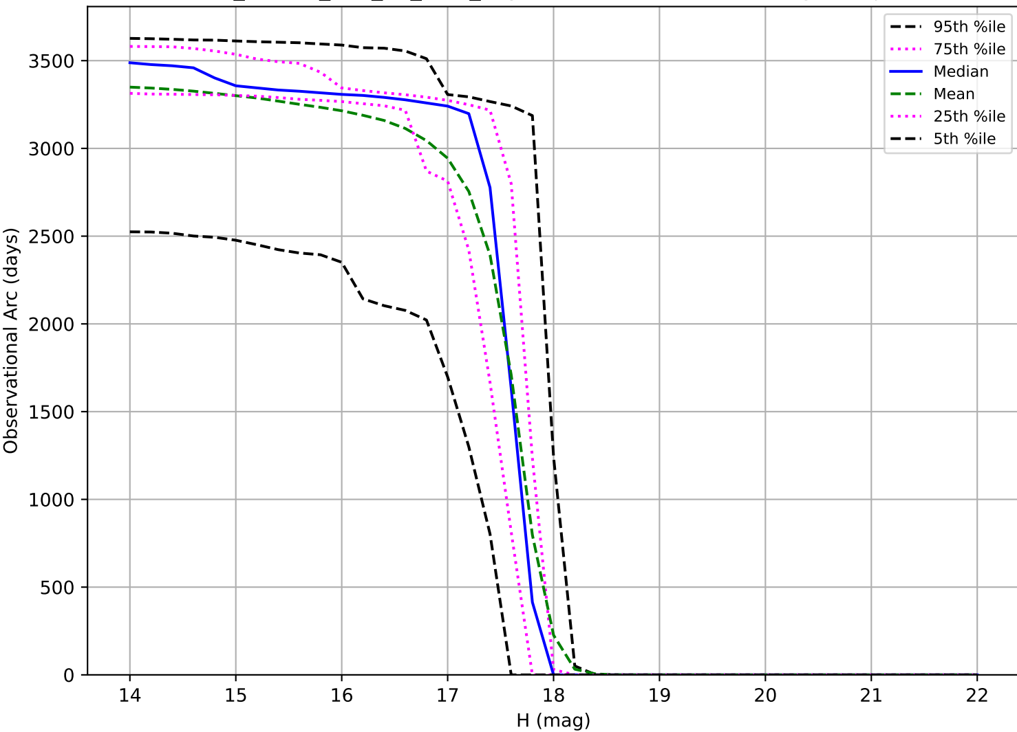
ddf_loaded_half_fl2_v3.4_10yrs: Observational Arc Length Trojan
