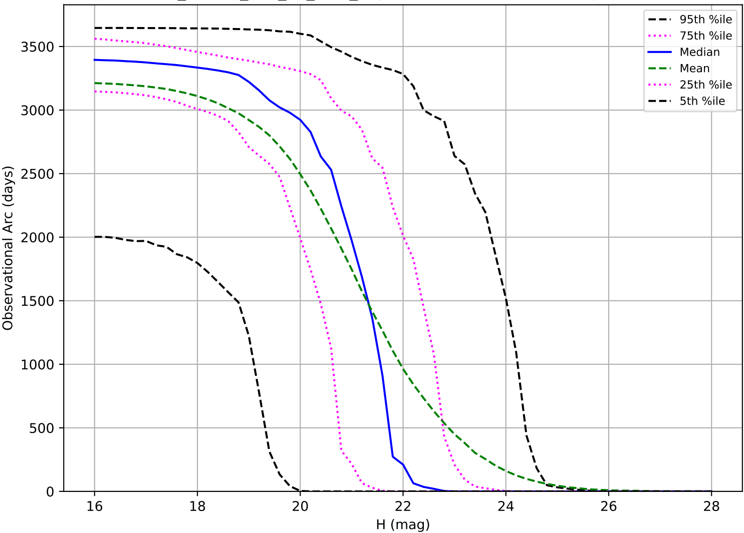
ddf_loaded_half_fl2_v3.4_10yrs: Observational Arc Length PHA
