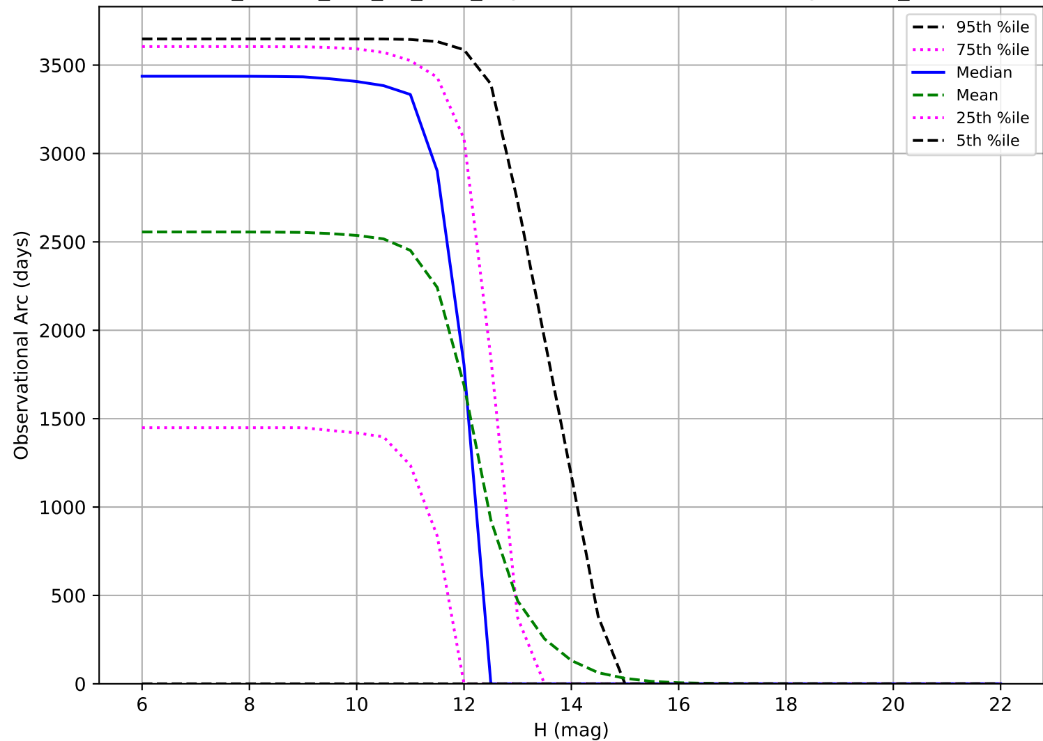
ddf_loaded_half_fl2_v3.4_10yrs: Observational Arc Length OCC_r20
