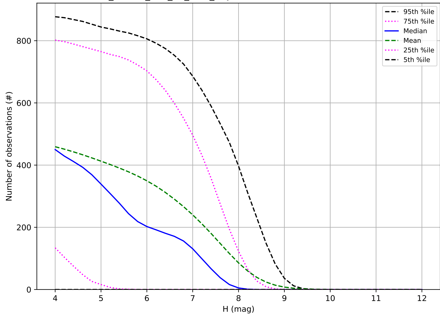
ddf_loaded_half_fl2_v3.4_10yrs: Number of observations TNO
