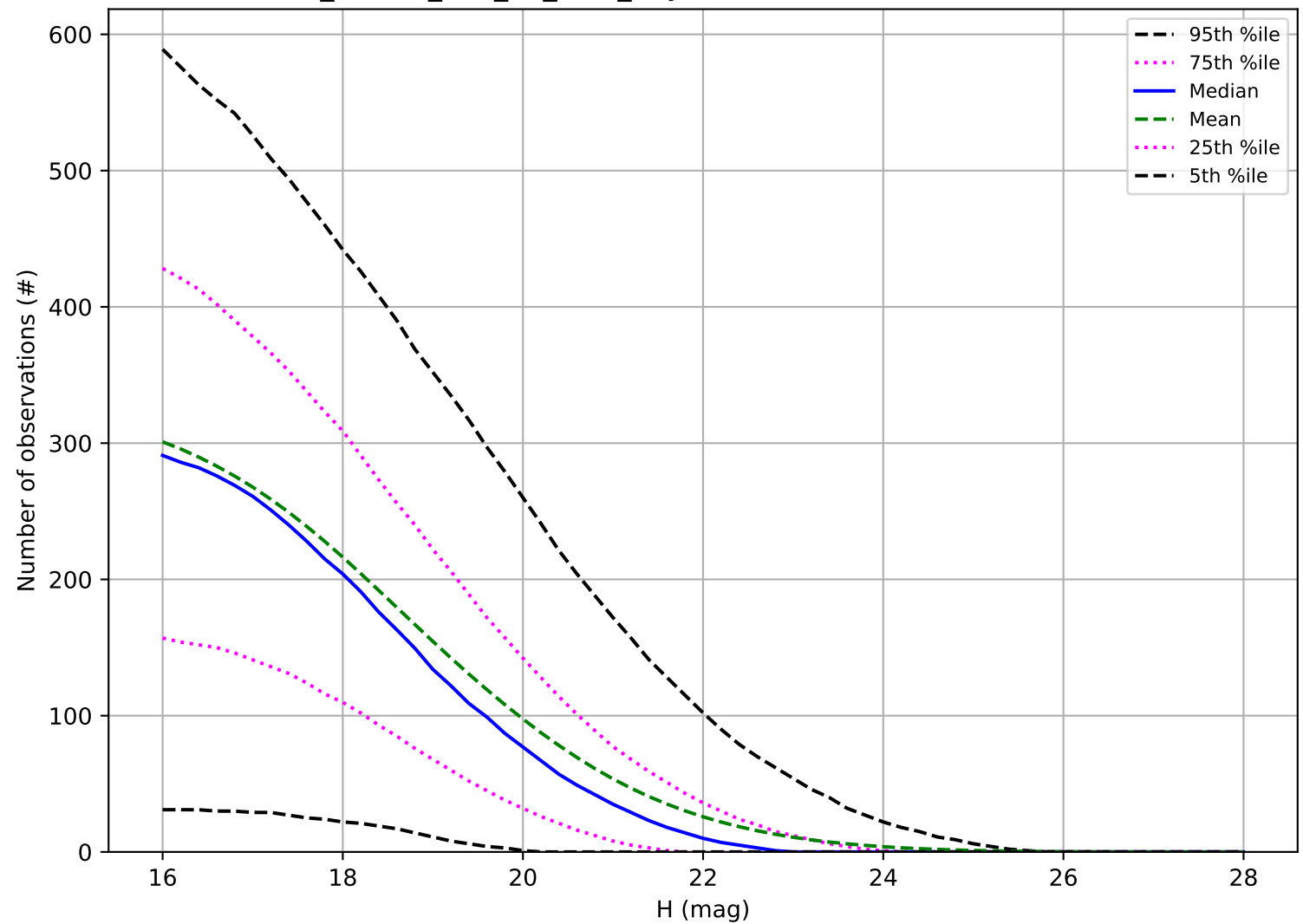
ddf_loaded_half_f12_v3.4_10yrs: Number of observations NEO
