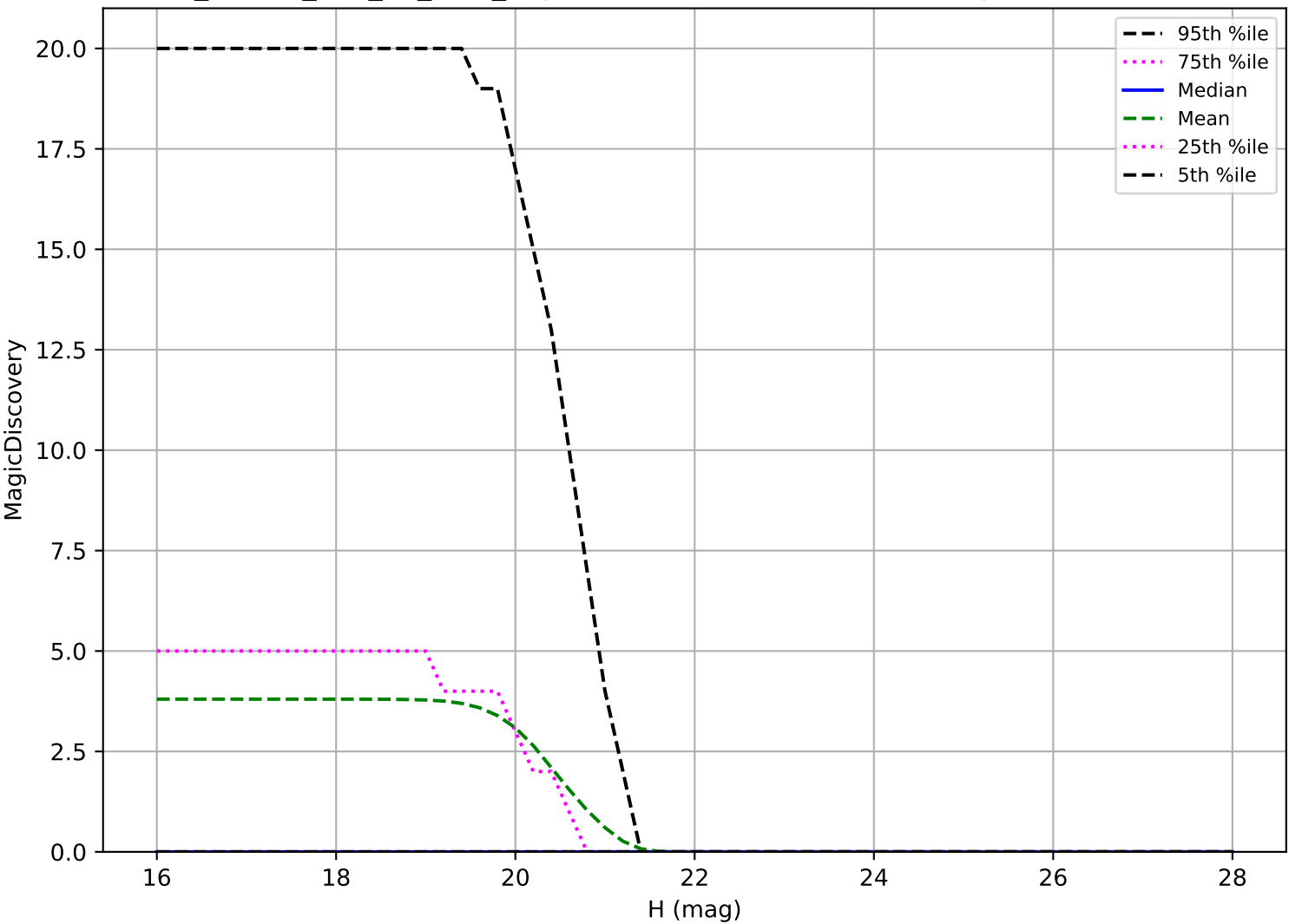
ddf_loaded_half_fl2_v3.4_10yrs: Vatira 6 detections in 60 nights detection loss
