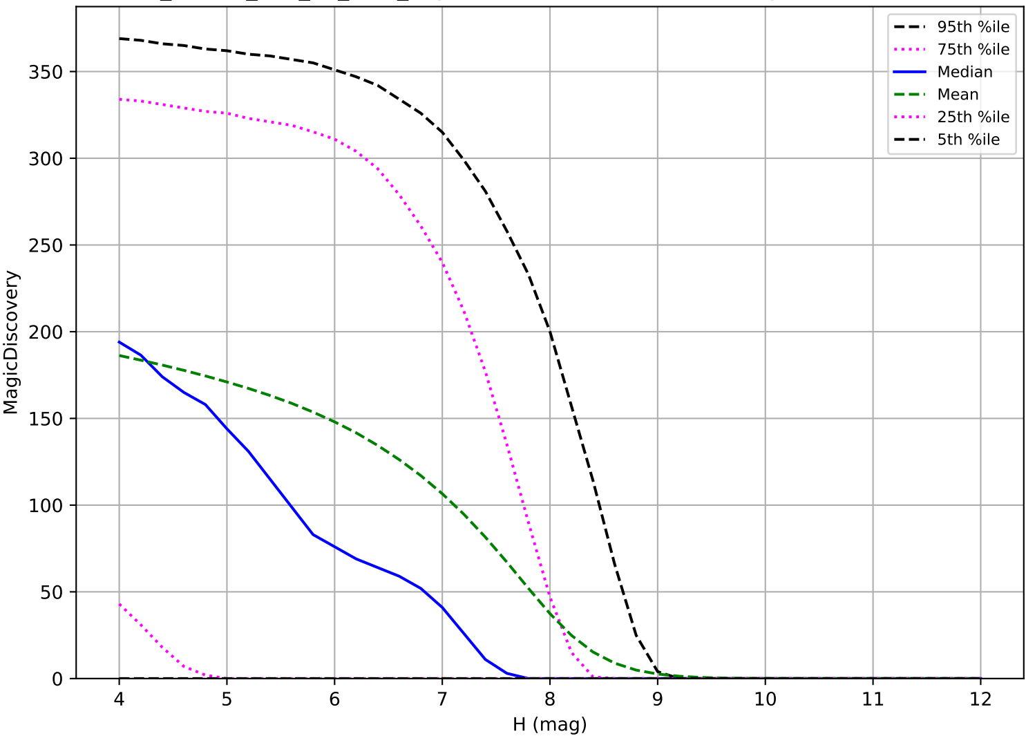
ddf_loaded_half_f12_v3.4_10yrs: TNO 6 detections in 60 nights detection loss
