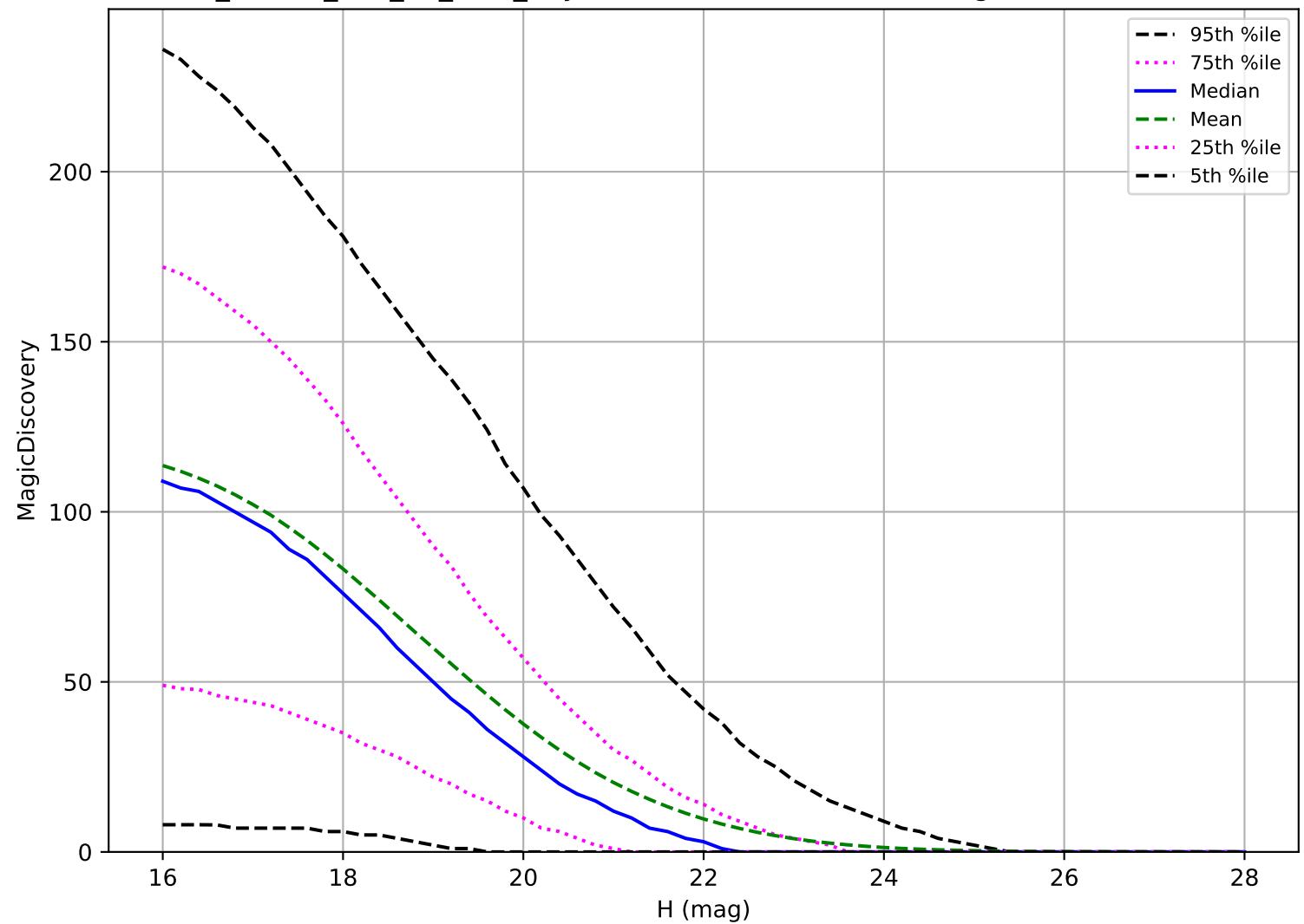
ddf_loaded_half_fl2_v3.4_10yrs: PHA 6 detections in 60 nights detection loss
