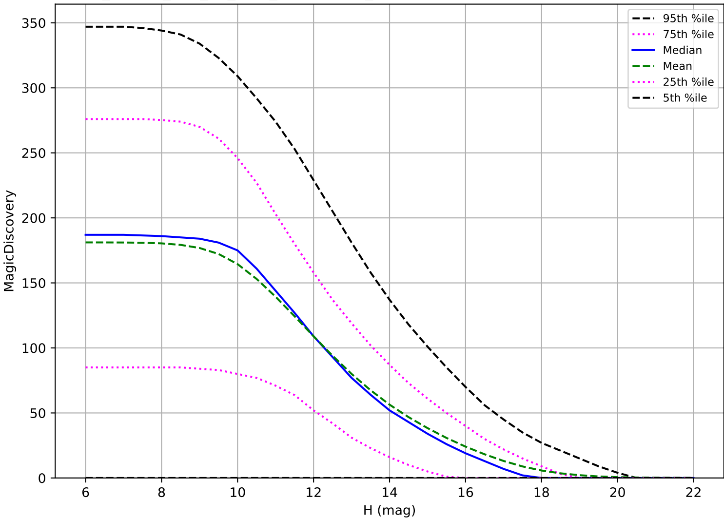
ddf_loaded_half_f12_v3.4_10yrs: OCC_r5 6 detections in 60 nights detection loss
