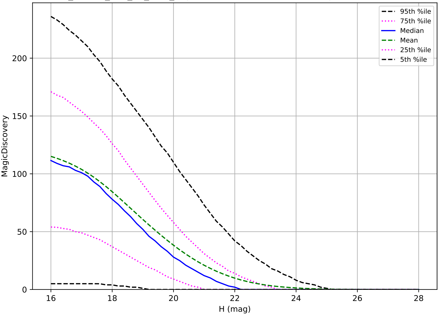
ddf_loaded_half_fl2_v3.4_10yrs: NEO 6 detections in 60 nights detection loss
