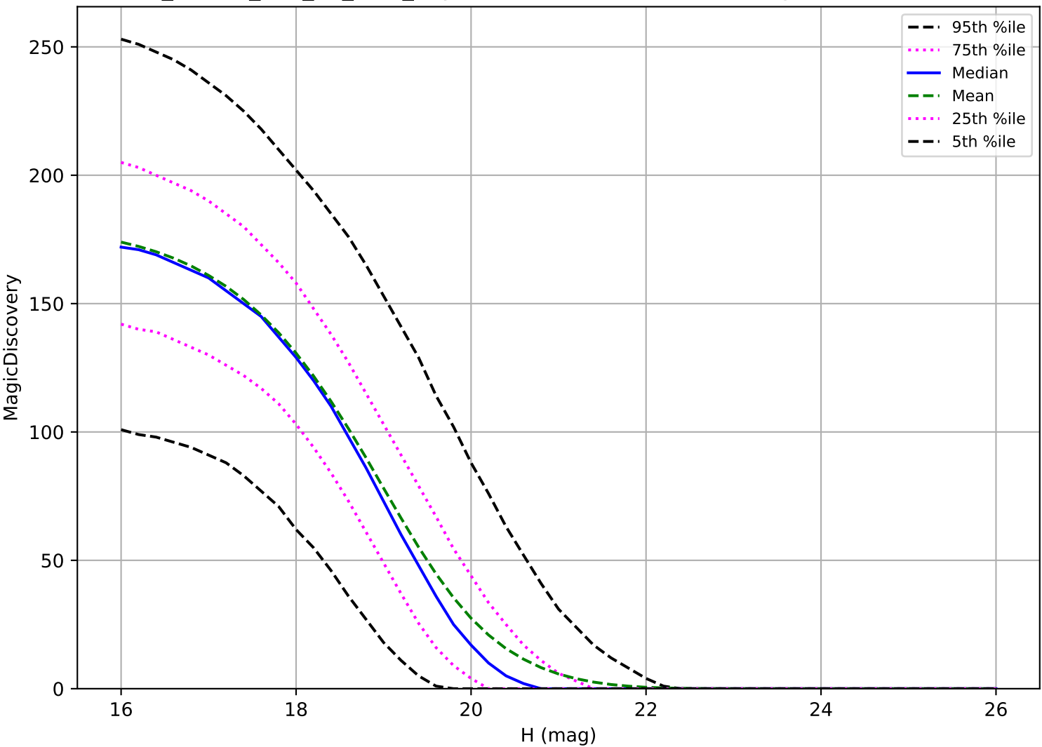
ddf_loaded_half_f12_v3.4_10yrs: MBA 6 detections in 60 nights detection loss
