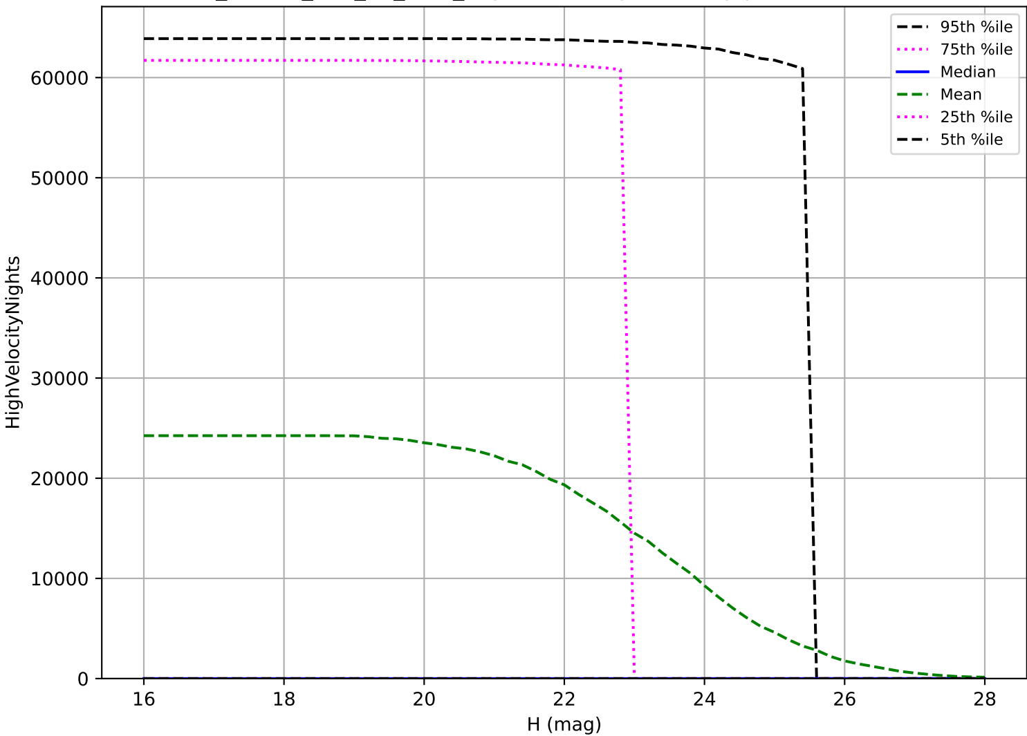
ddf_loaded_half_f12_v3.4_10yrs: PHA High velocity pair detection loss
