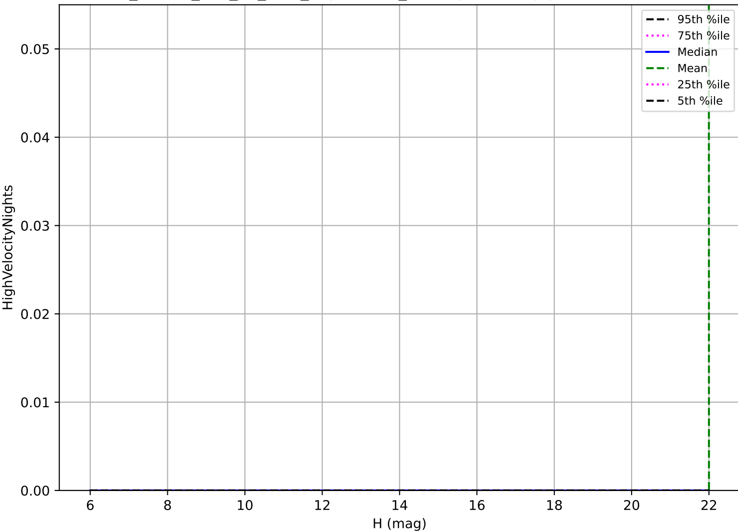
ddf_loaded_half_fl2_v3.4_10yrs: OCC_r20 High velocity pair detection loss
