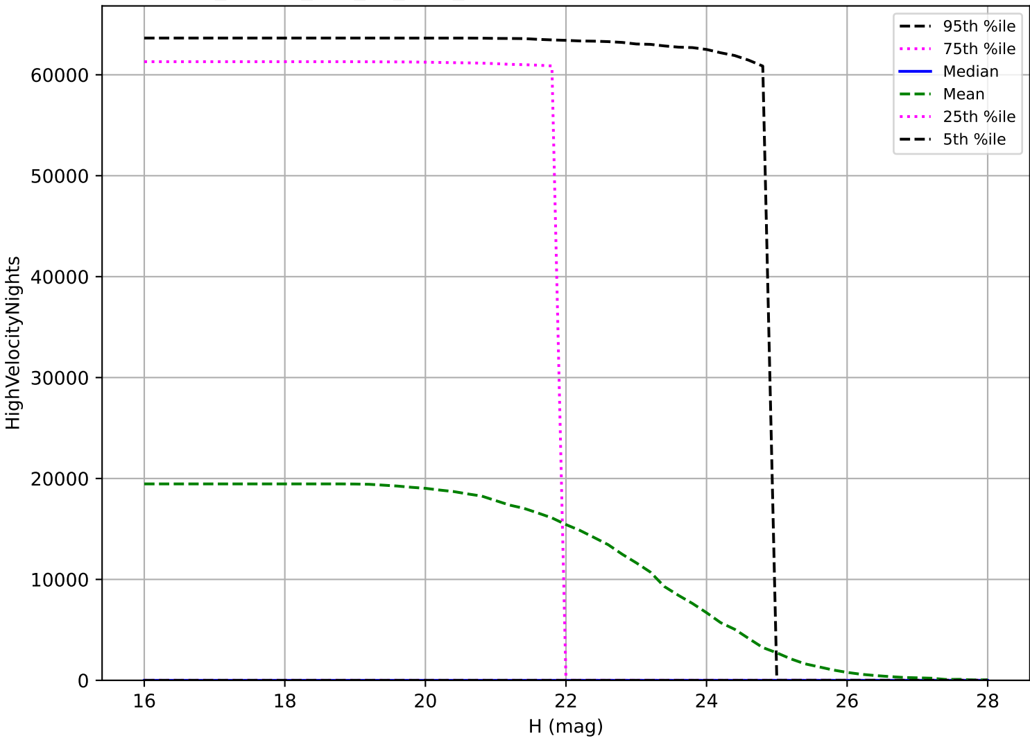
ddf_loaded_half_f12_v3.4_10yrs: NEO High velocity pair detection loss
