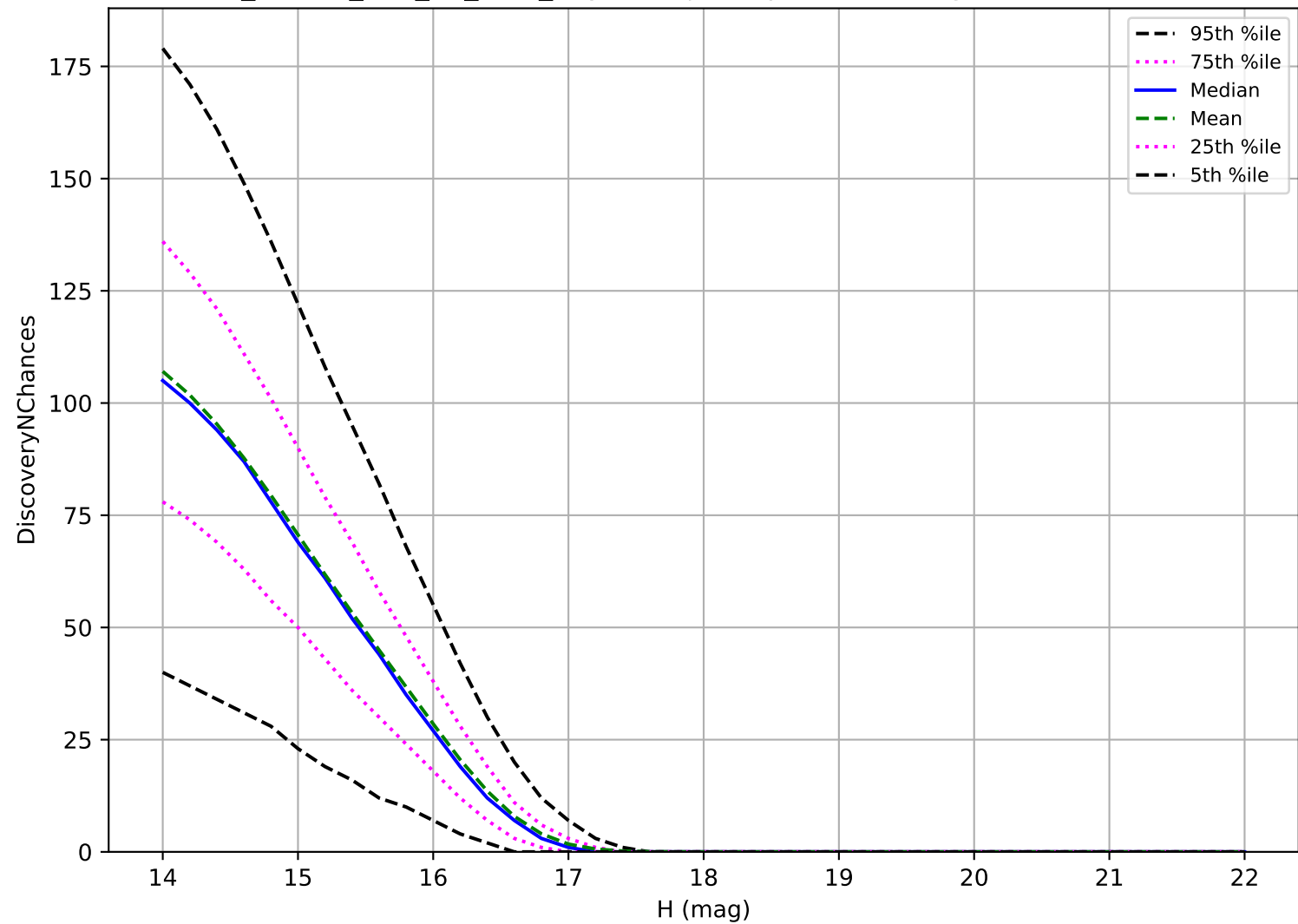
ddf_loaded_half_fl2_v3.4_10yrs: Trojan 3 pairs in 15 nights detection loss
