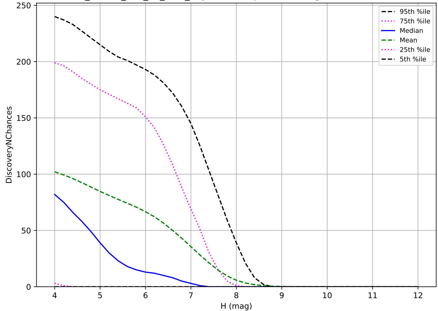
ddf_loaded_half_fl2_v3.4_10yrs: TNO 3 pairs in 15 nights detection loss
