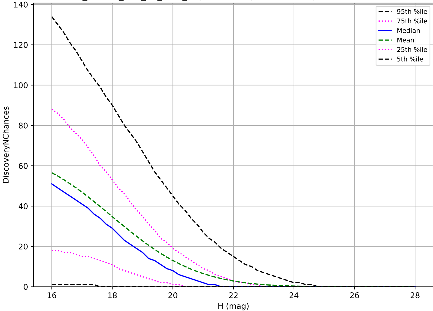
ddf_loaded_half_f12_v3.4_10yrs: PHA 3 pairs in 15 nights detection loss
