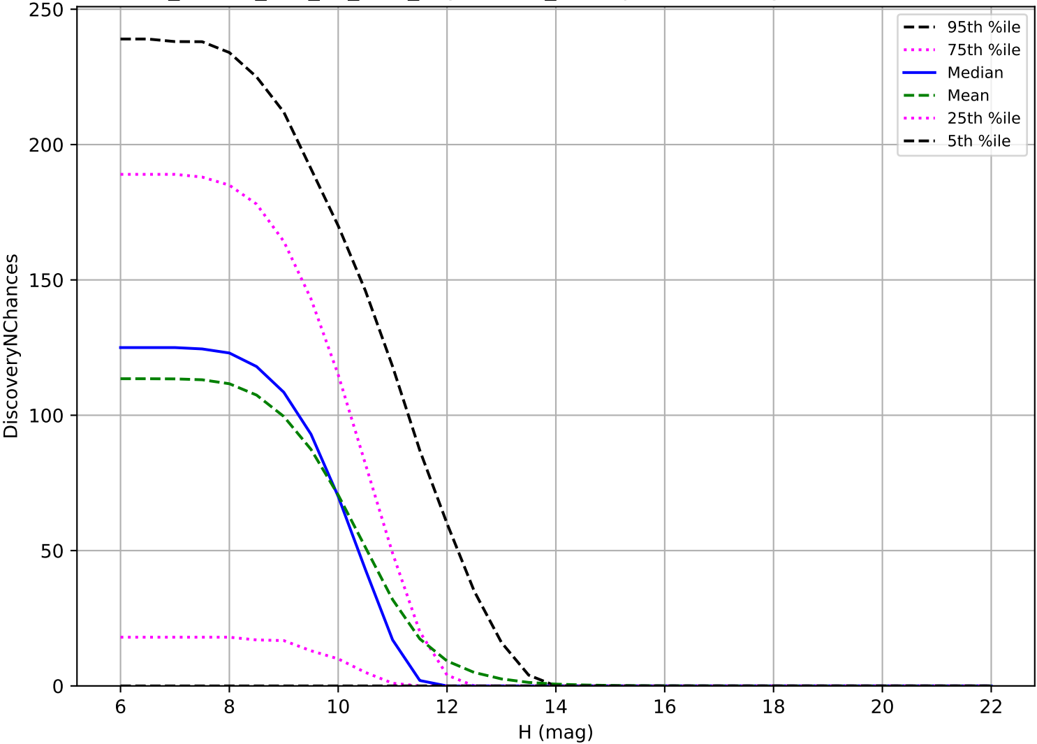
ddf_loaded_half_f12_v3.4_10yrs: OCC_r20 3 pairs in 15 nights detection loss
