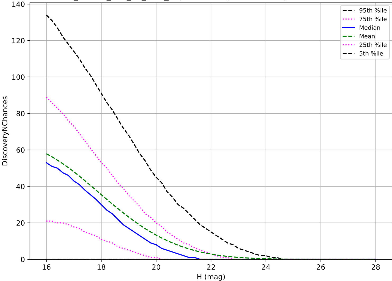
ddf_loaded_half_f12_v3.4_10yrs: NEO 3 pairs in 15 nights detection loss
