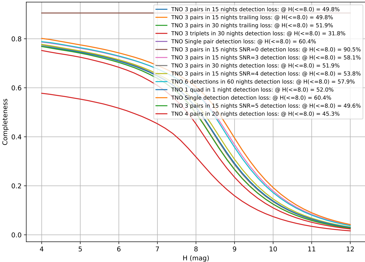
ddf_loaded_half_fl2_v3.4_10yrs: CumulativeCompleteness
