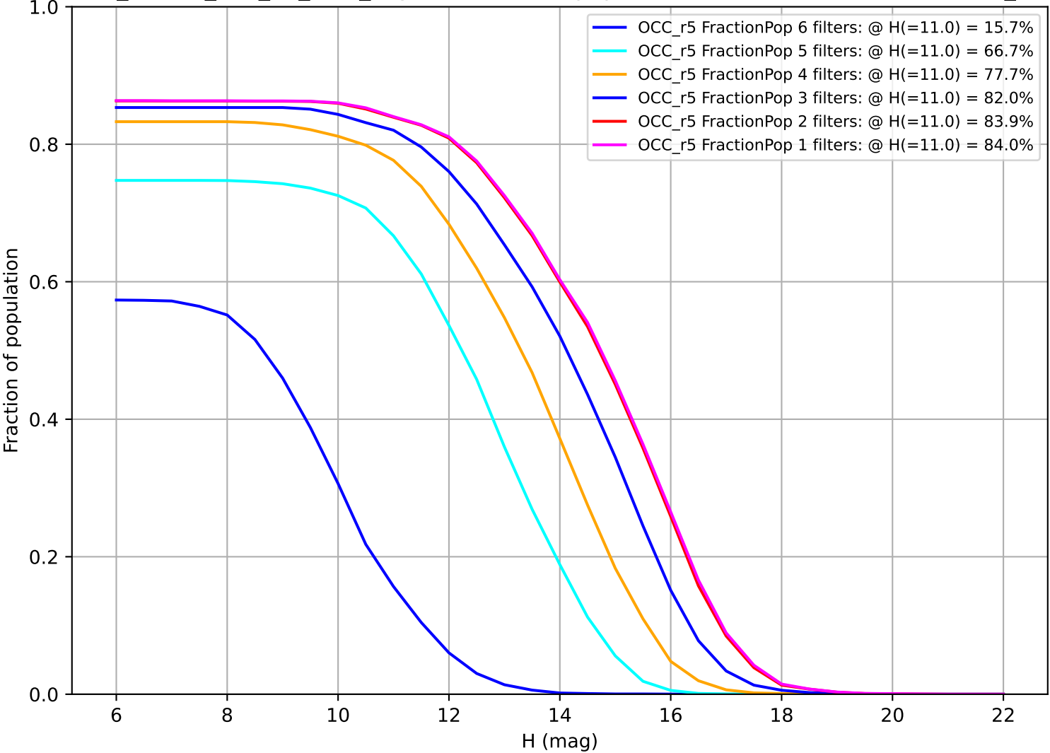
ddf_loaded_half_fl2_v3.4_10yrs: Fraction of population with colors in X filters OCC_r5
