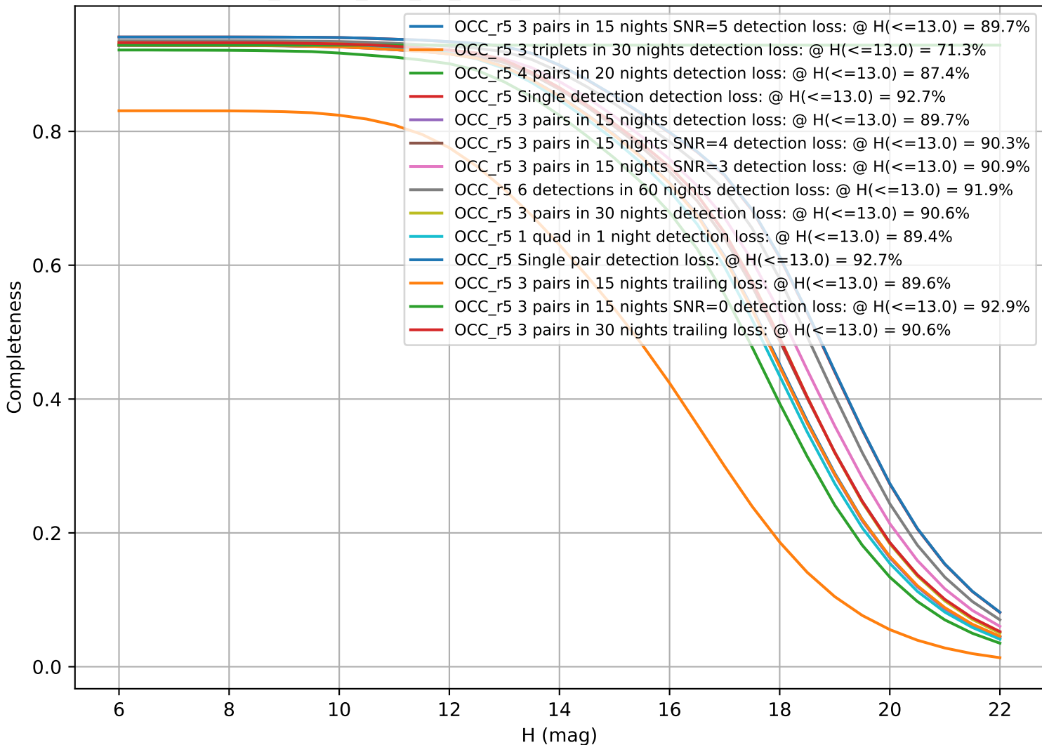
ddf_loaded_half_fl2_v3.4_10yrs: CumulativeCompleteness
