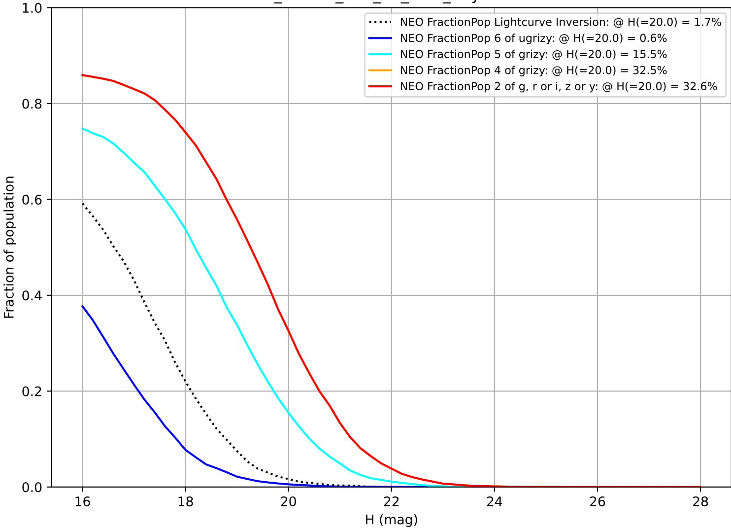
ddf_loaded_half_fl2_v3.4_10yrs NEO
