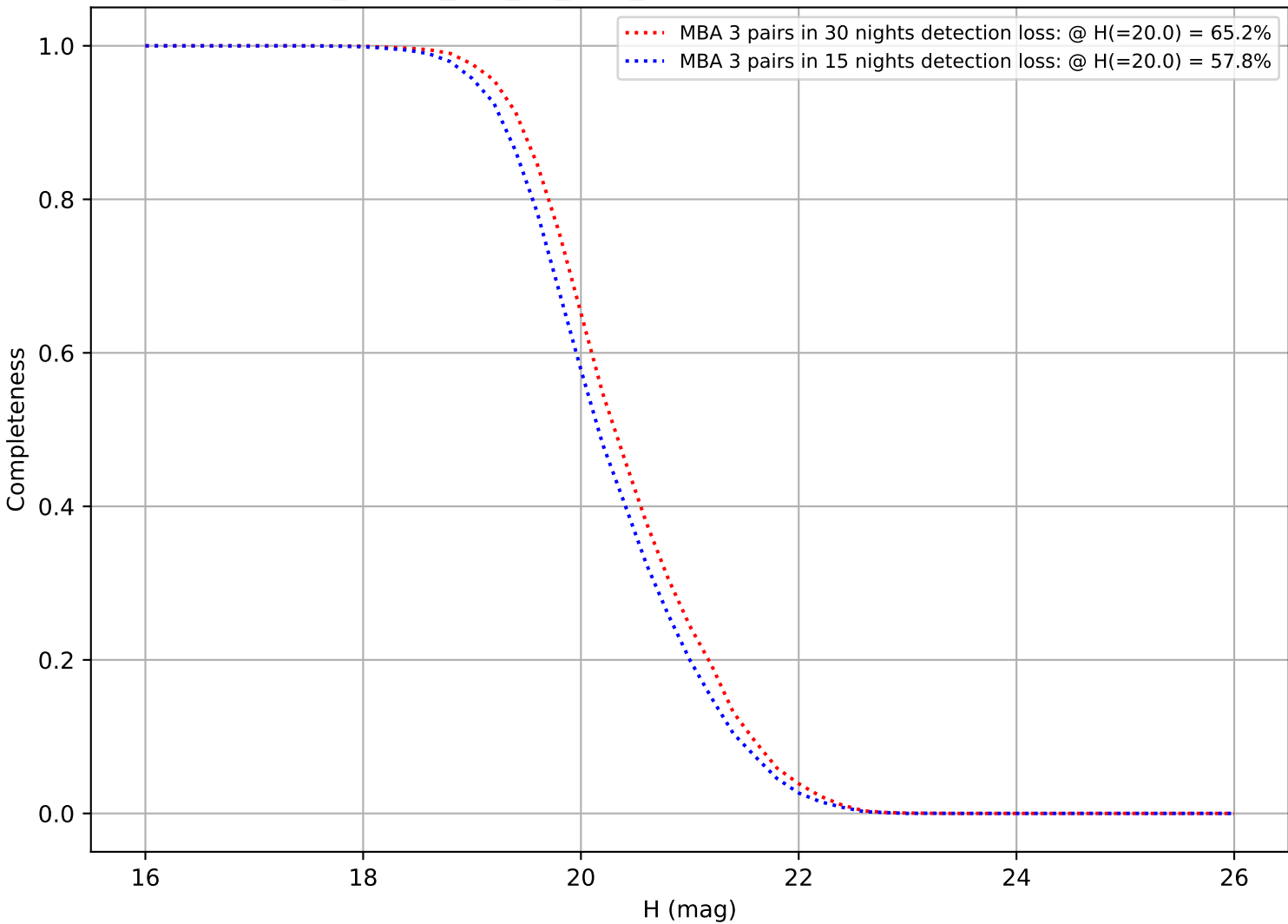
ddf_loaded_half_f12_v3.4_10yrs: DifferentialCompleteness
