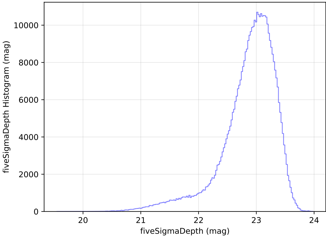
ddf_loaded_half_fl2_v3.4_10yrs z: fiveSigmaDepth Histogram
