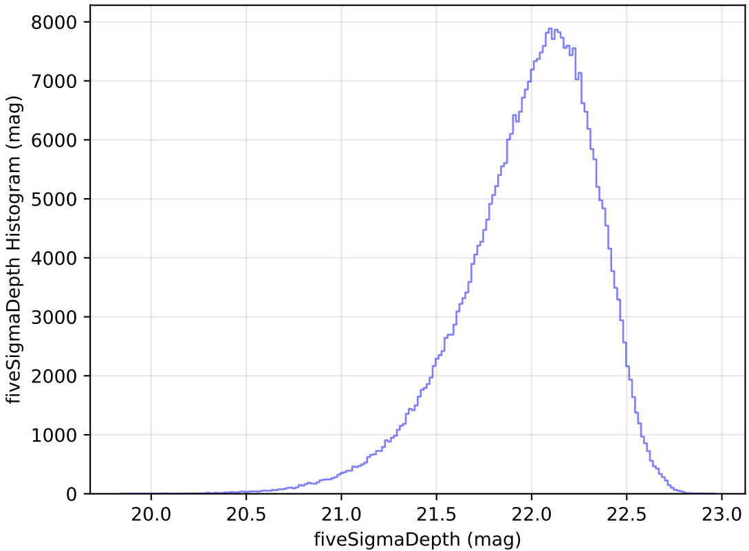
ddf_loaded_half_fl2_v3.4_10yrs y: fiveSigmaDepth Histogram
