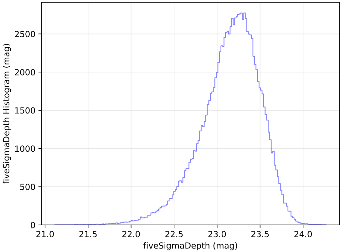
ddf_loaded_half_fl2_v3.4_10yrs u: fiveSigmaDepth Histogram
