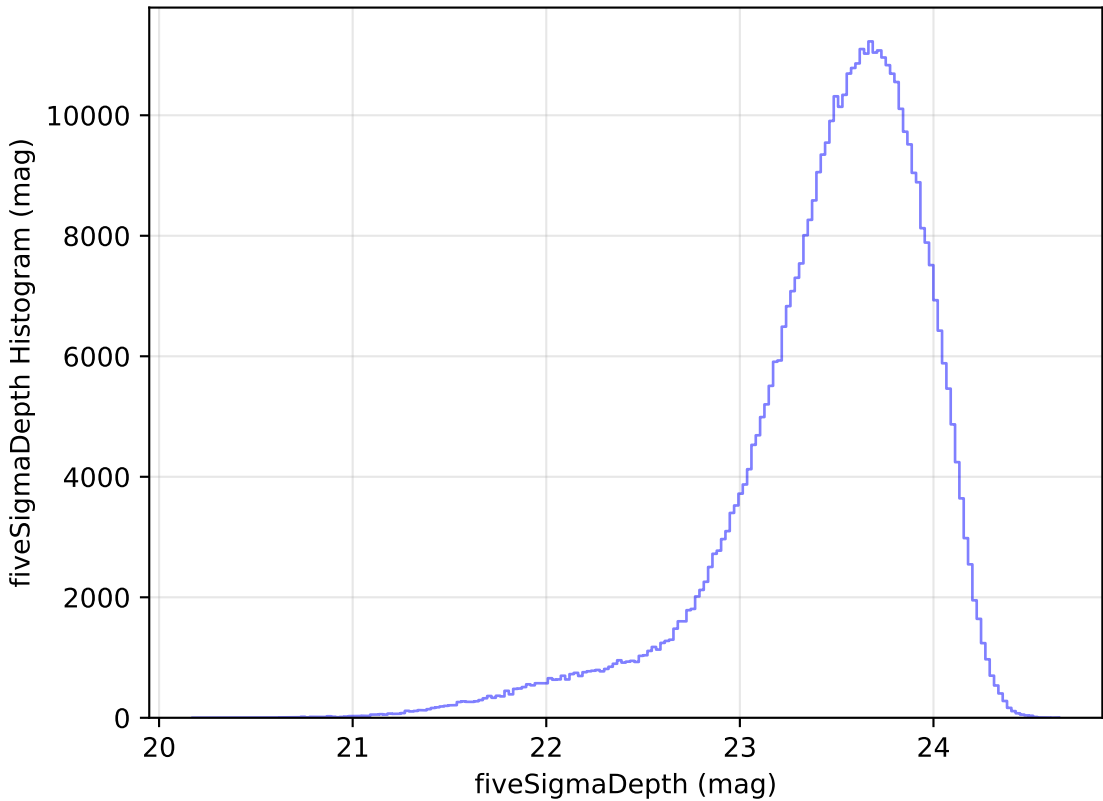
ddf_loaded_half_fl2_v3.4_10yrs i: fiveSigmaDepth Histogram
