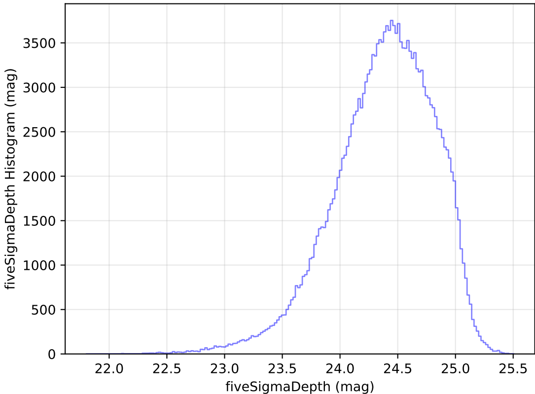
ddf_loaded_half_fl2_v3.4_10yrs g: fiveSigmaDepth Histogram
