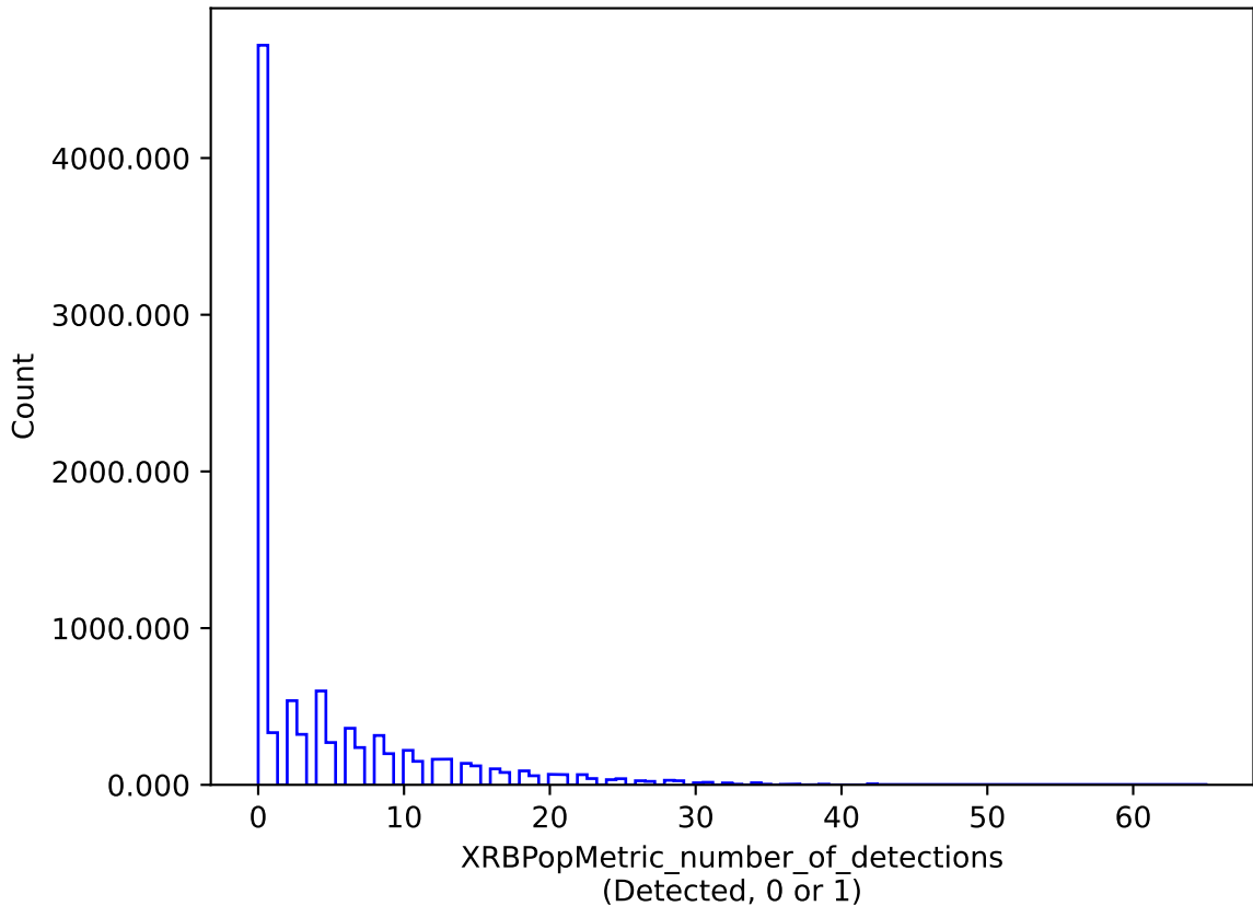
ddf_loaded_half_fl2_v3.4_10yrs : XRBPoMetric_number_of_detections
