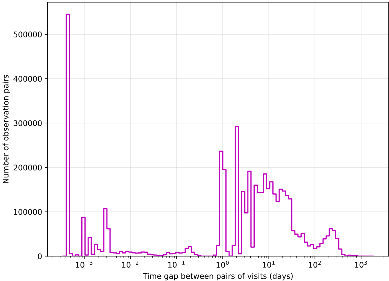
ddf_loaded_half_fl2_v3.4_10yrs z band: Tgaps observationStartMJD
