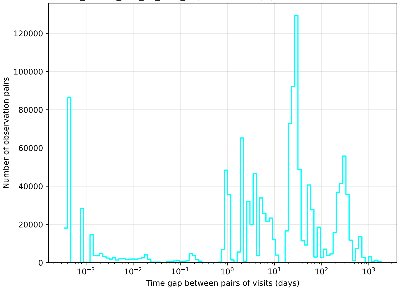
ddf_loaded_half_fl2_v3.4_10yrs u band: Tgaps observationStartMJD
