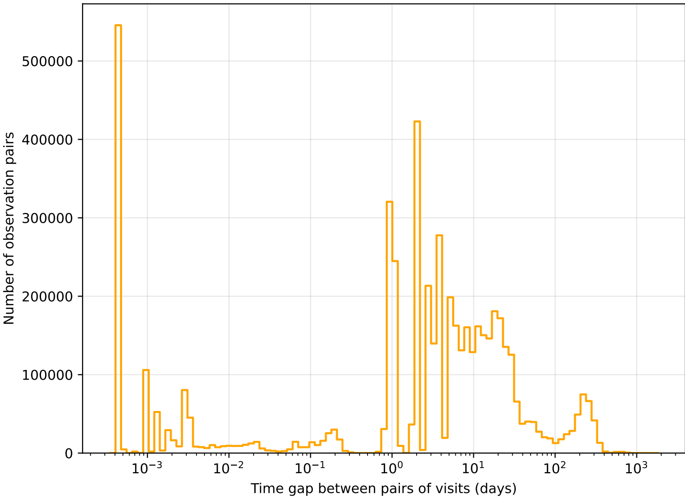
ddf_loaded_half_f12_v3.4_10yrs r band: Tgaps observationStartMJD
