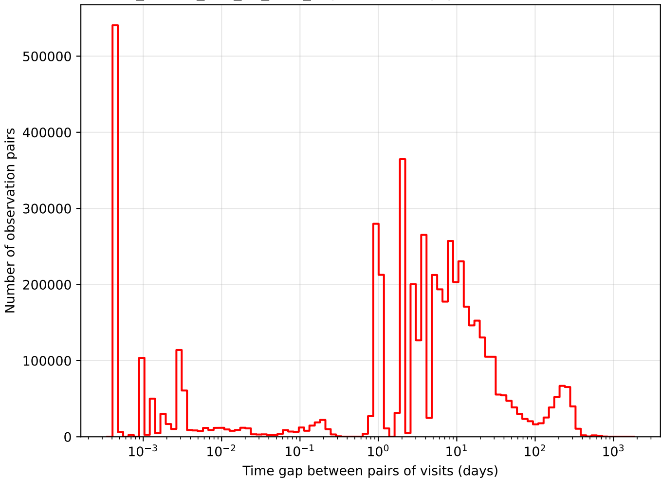
ddf_loaded_half_fi2_v3.4_10yrs i band: Tgaps observationStartMJD
