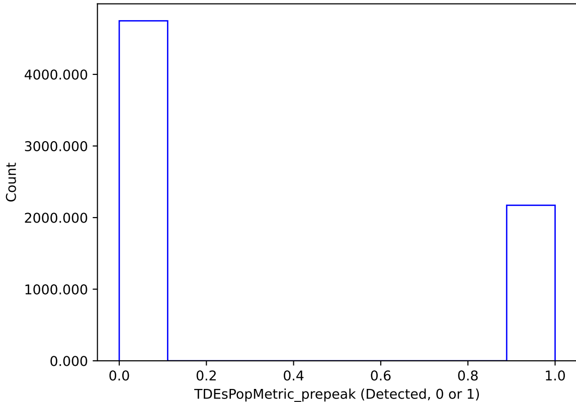
ddf_loaded_half_fl2_v3.4_10yrs : TDEsPopMetric_prepeak
