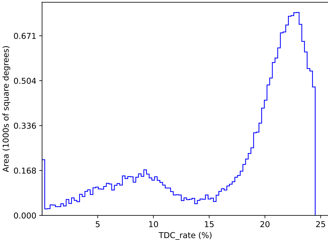
ddf_loaded_half_fl2_v3.4_10yrs : TDC_rate
