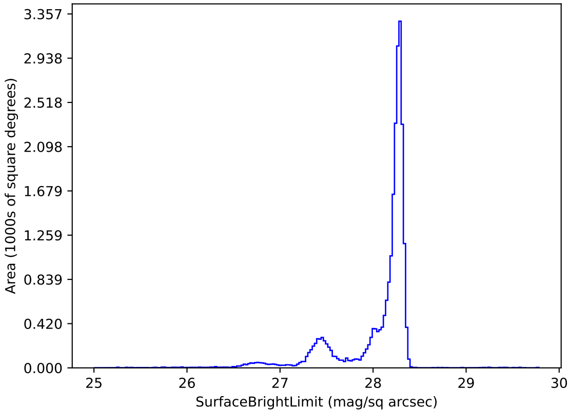
ddf_loaded_half_fl2_v3.4_10yrs y: SurfaceBrightLimit
