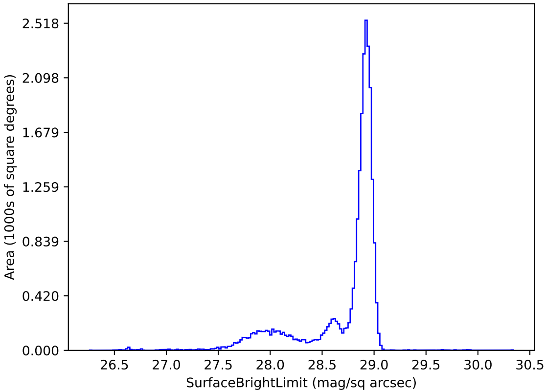
ddf_loaded_half_fl2_v3.4_10yrs u: SurfaceBrightLimit
