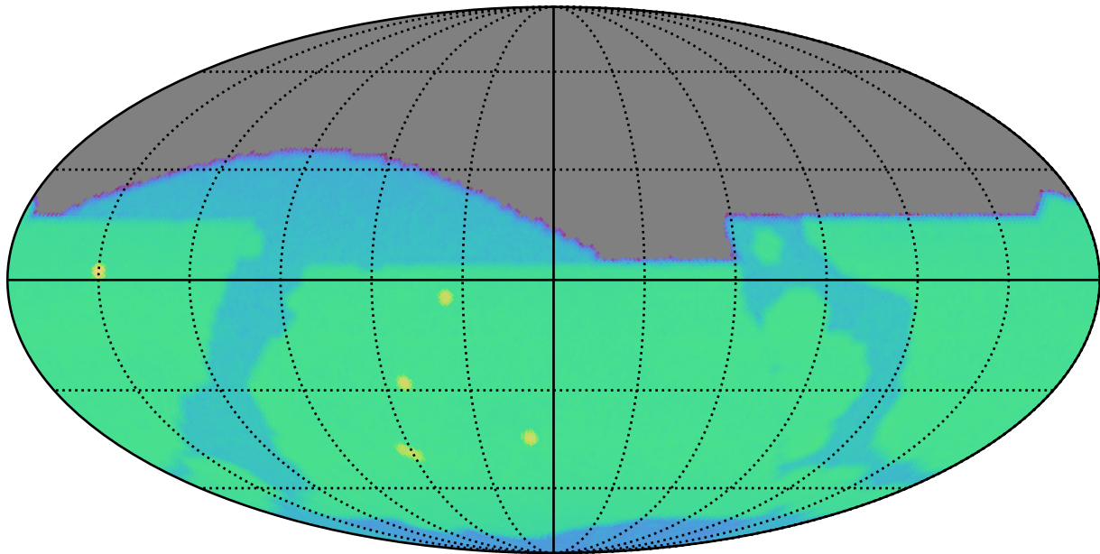
ddf_loaded_half_fl2_v3.4_10yrs i: SurfaceBrightLimit
