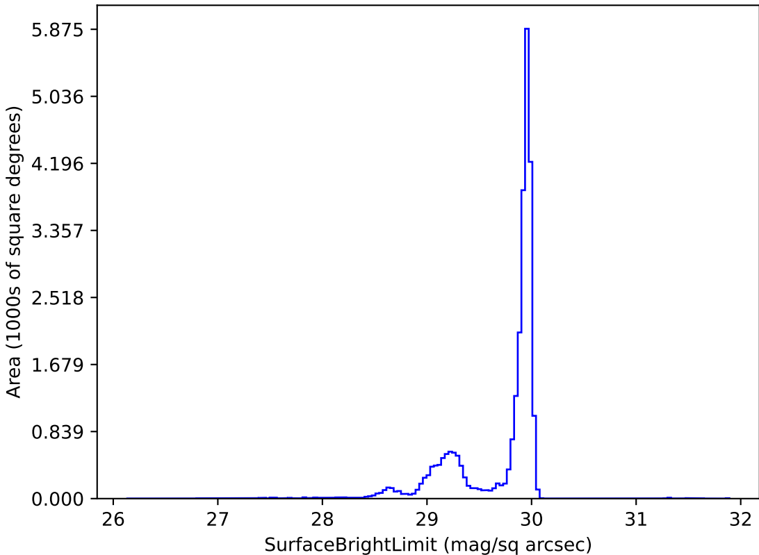
ddf_loaded_half_fl2_v3.4_10yrs i: SurfaceBrightLimit
