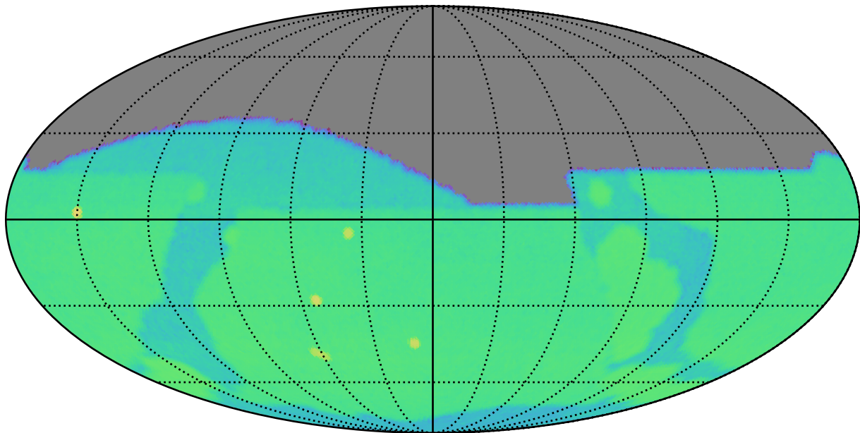
ddf_loaded_half_fl2_v3.4_10yrs g: SurfaceBrightLimit
