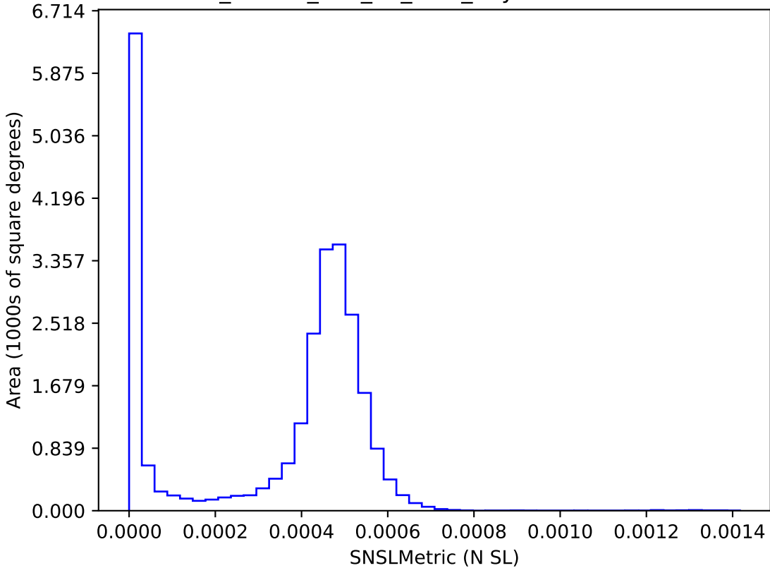
ddf_loaded_half_fl2_v3.4_10yrs : SNSLMetric
