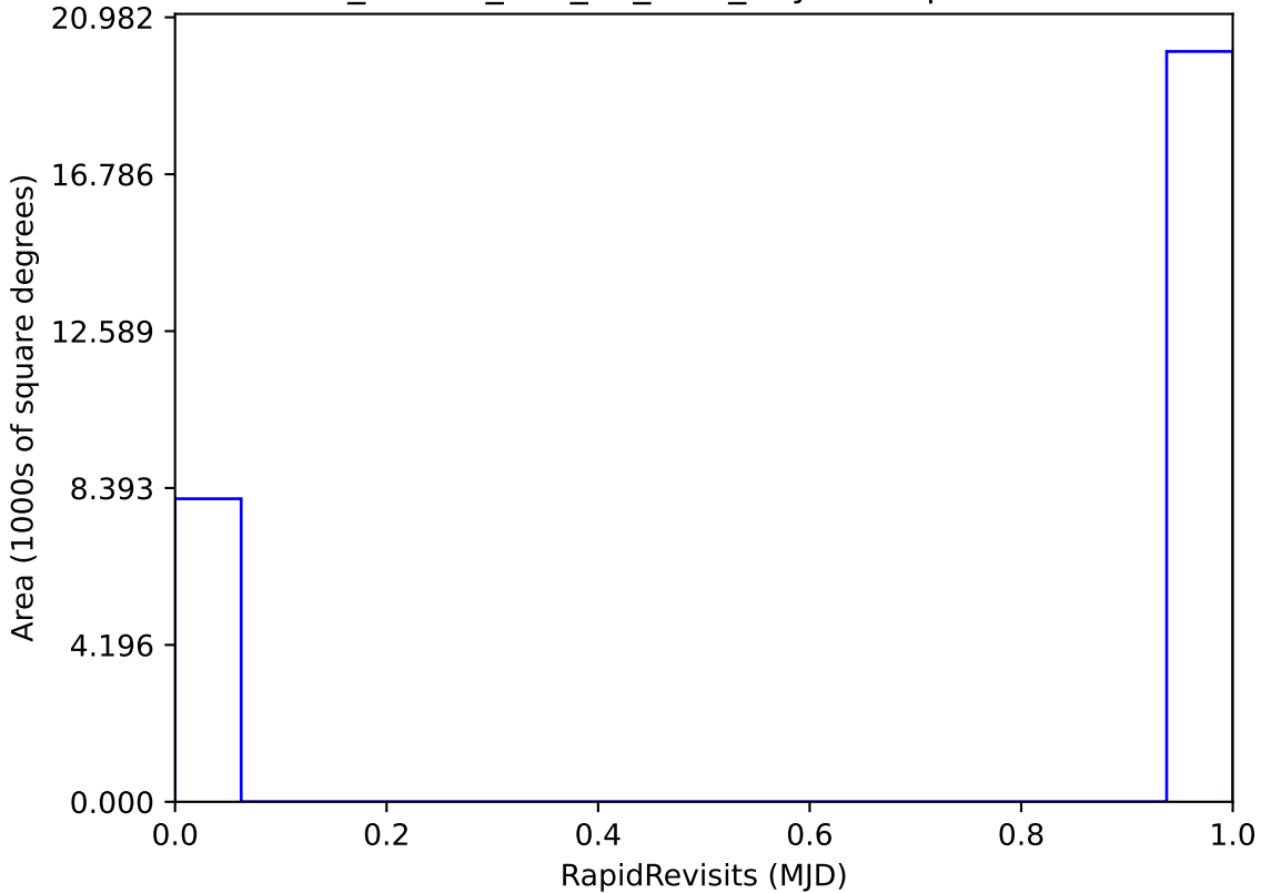
ddf_loaded_half_fl2_v3.4_10yrs : RapidRevisits
