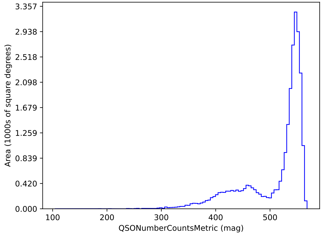
ddf_loaded_half_f12_v3.4_10yrs i band and non-DD: QSONumberCountsMetric
